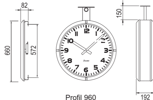
Profil 960 single or double face
